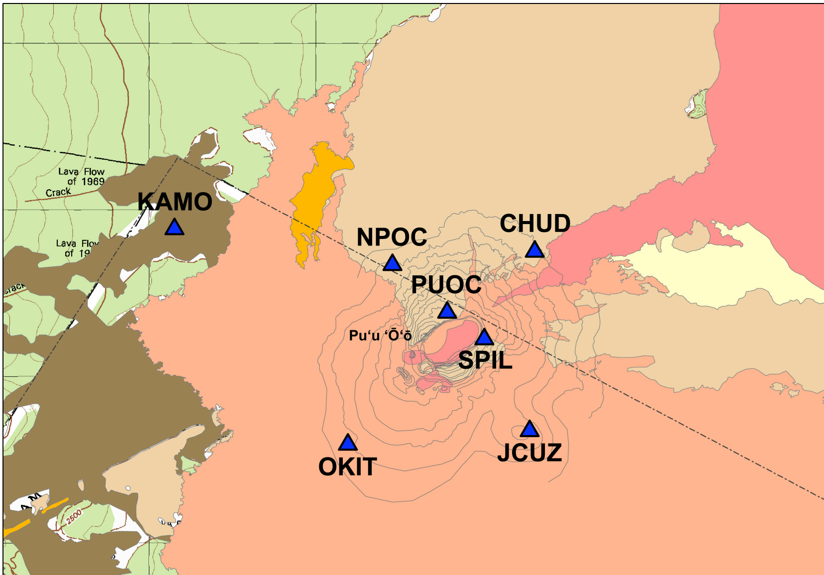
Map of the GPS network near Pu'u 'Ō'ō. Base map colors correspond to different lava flow ages. See the History section at VEPP website for more information.
